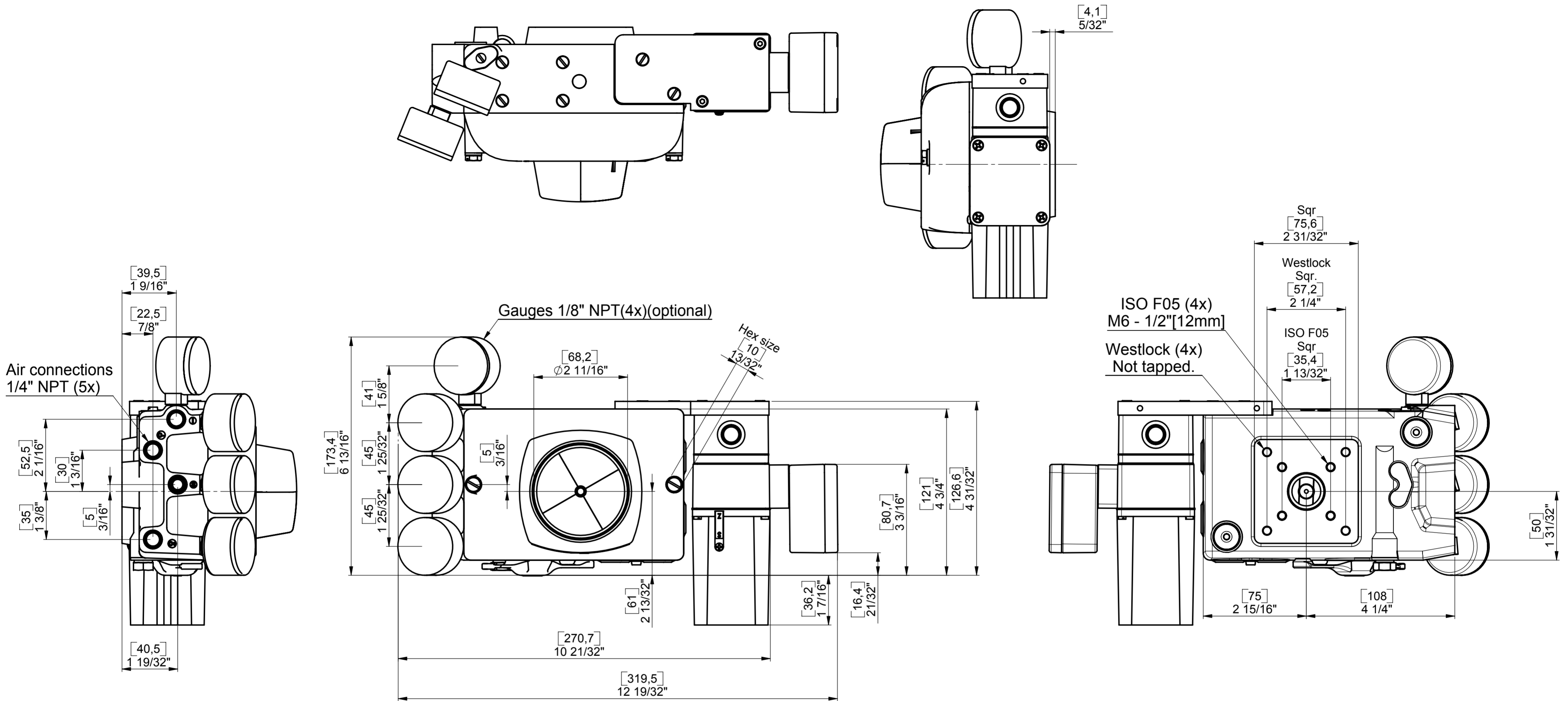
Dimensional Drawing VAC Positioner V200 FF IP-WatsonSmith 420 Fail Freeze
