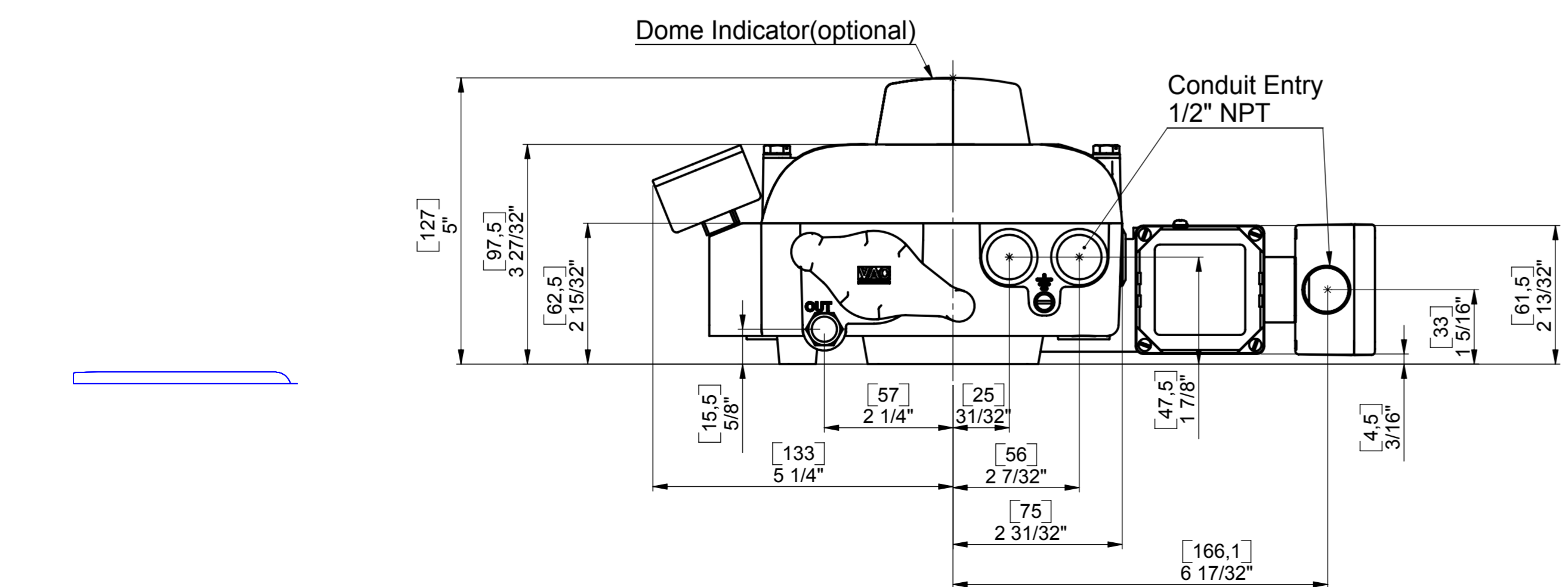
Dimensional Drawing VAC Positioner V200 FF IP-WatsonSmith 420 Fail Freeze
